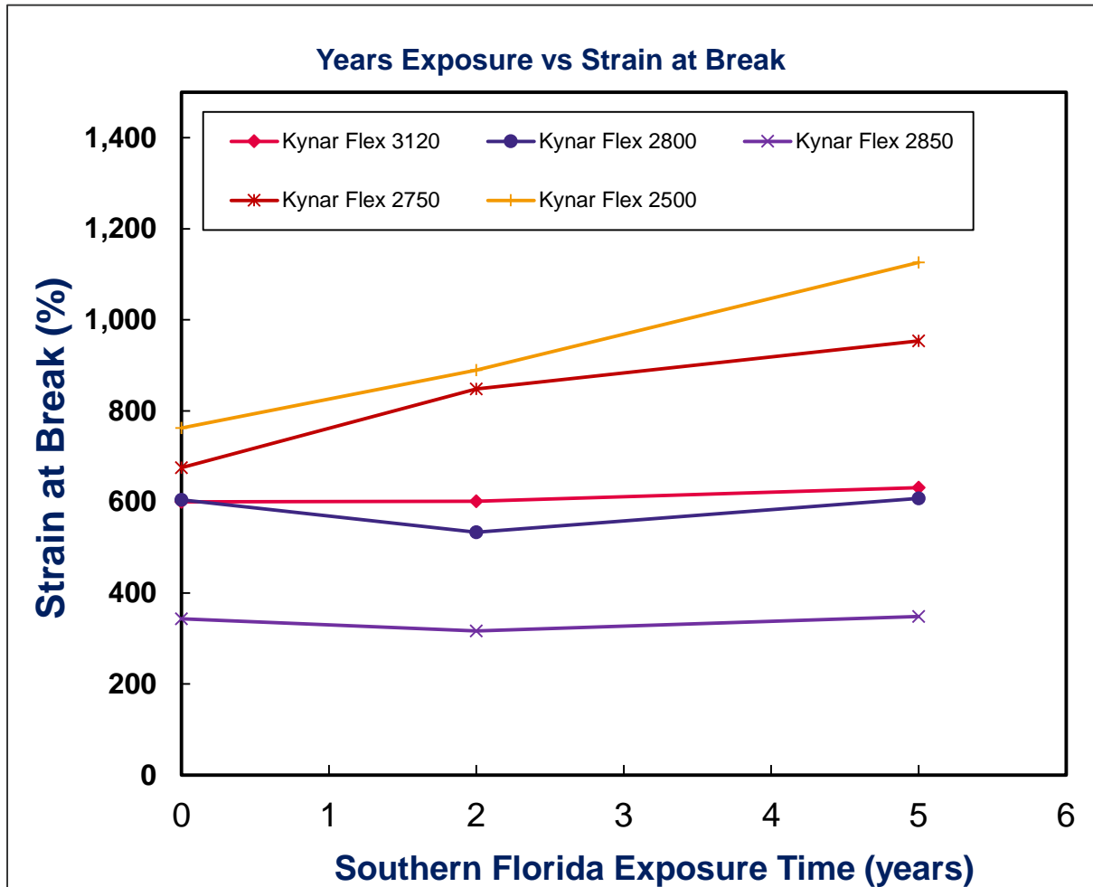
Five years in S. Florida – total UV exposure calculated at 1600 MJ/m 2
