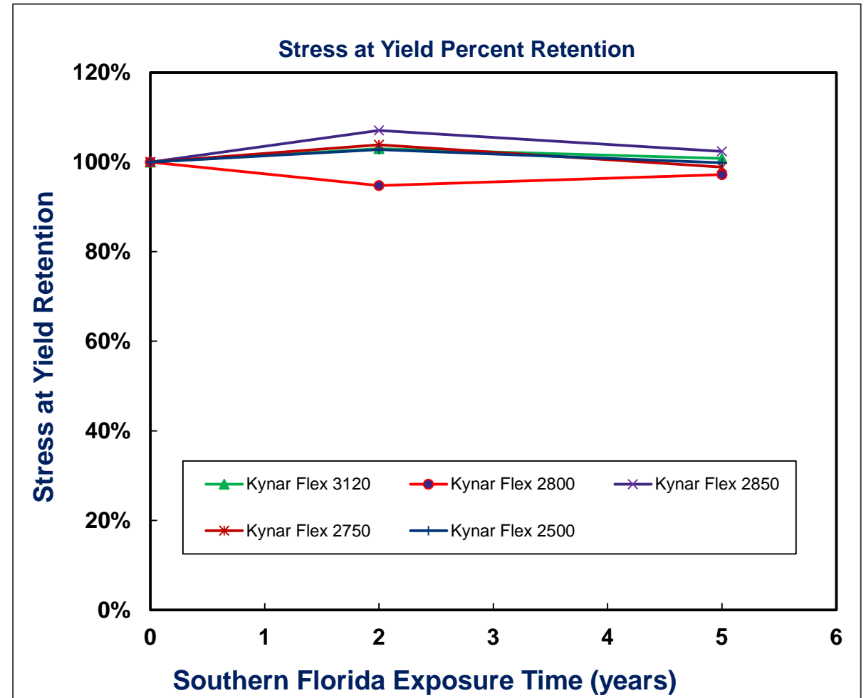
Film Thickness: 50 microns – except Kynar® 2500 and Kynar® 2750 at 125 microns
